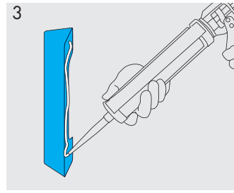
3 Apply mounting adhesive to the cut element.
