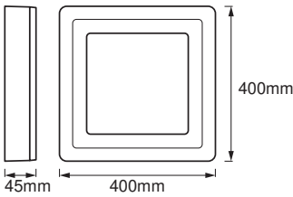
LED COLOR WHITE SQ 400mm 42W OSRAM
