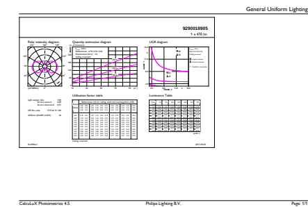
General uniform lighting - CorePro LEDLusterND4.3-40W E27 827P45CLG
