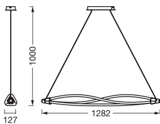
DECOR SWIRL PEND 22W 830 CLICK DIM
