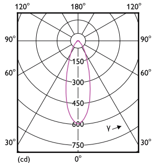
Light Distribution Diagram - CorePro LEDspot 4-50W GU10 830 36D DIM
