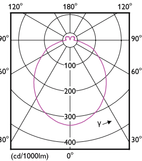
Light Distribution Diagram – Corepro LEDspot 550lm GU10 865 120D
